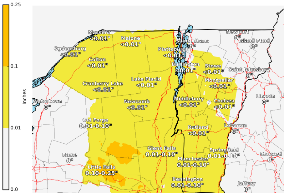
Expected Ice Accumulation- Official NWS Forecast Valid: 7 PM Friday January 01, 2021 to 7 PM Saturday January 02, 2021
